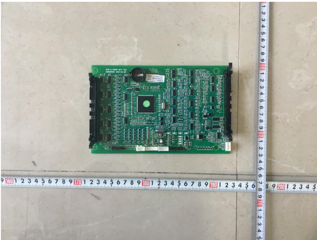
Front view of Control Board
