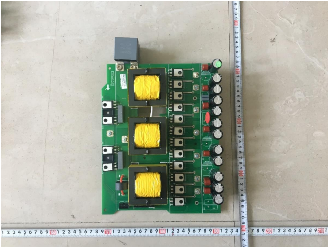
Front view of BOOST Board
